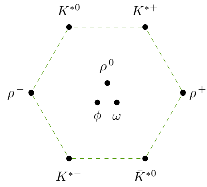
Vector Meson Nonet (Octet plus Singlet \omega )
